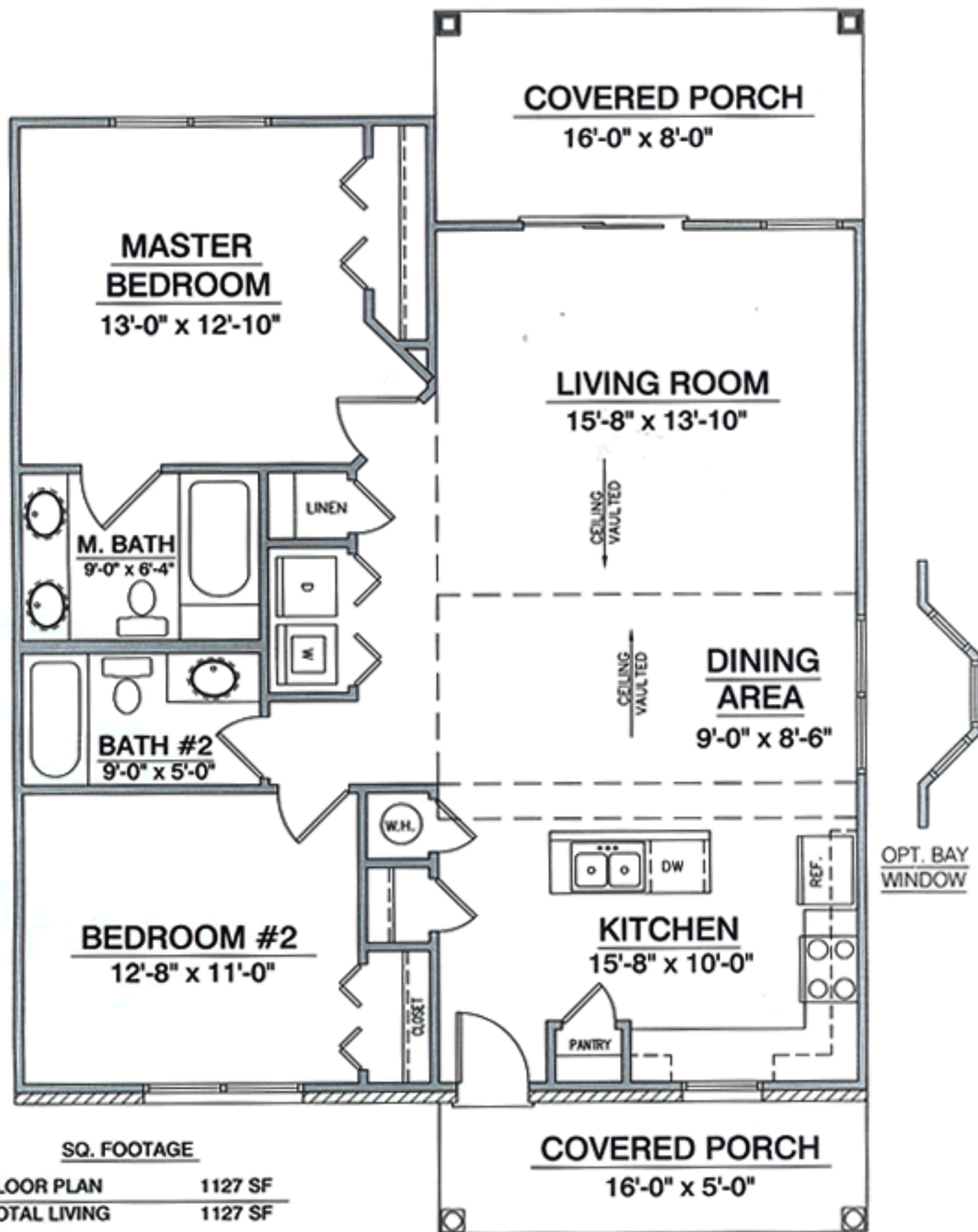
FLOOR PLAN
